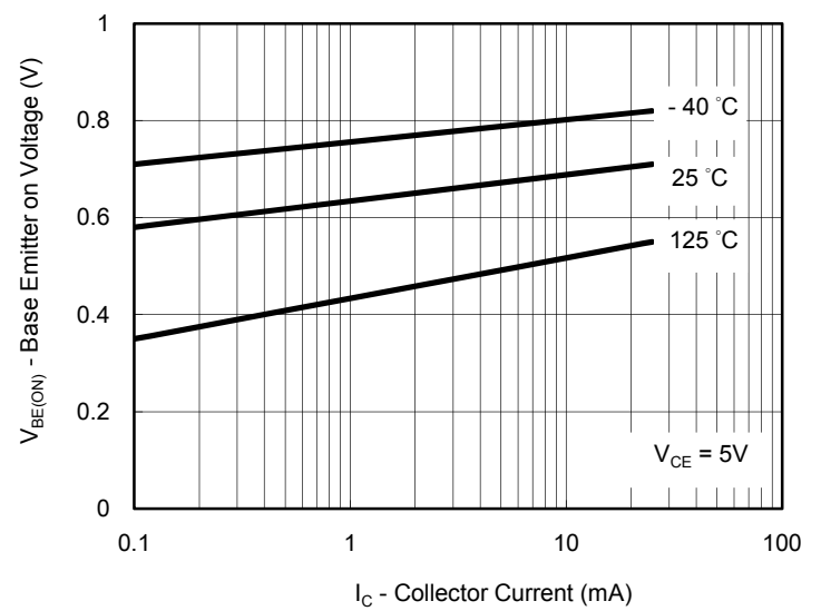
Fig. 4 Base Emitter On Voltage VS. Collector Current
